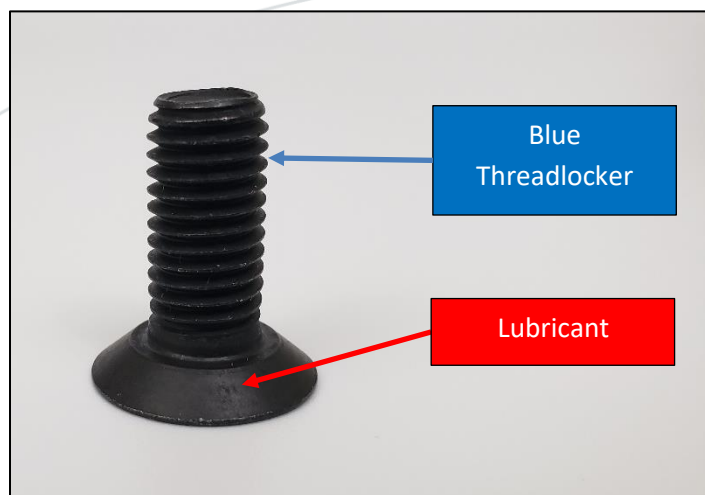
Figure 23: Countersink Bolts
