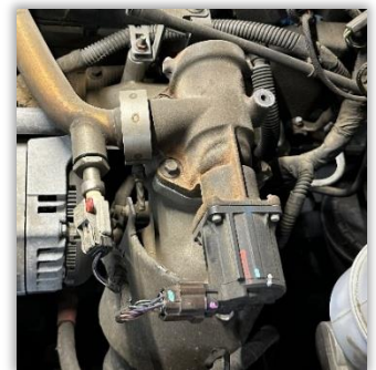
Figure 47: Example image of EGR Valve electrical connector and crossover tube temperature sensor, reinstalled.
