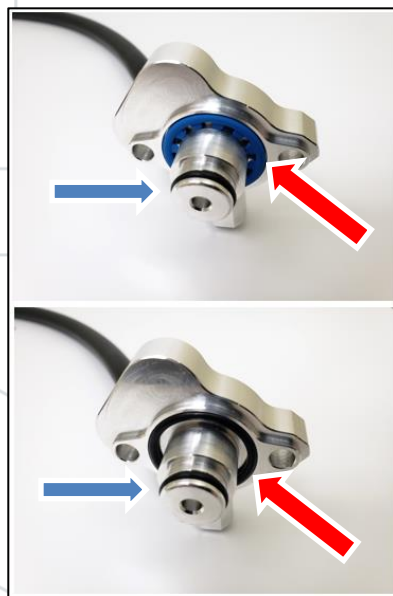
Figure 10: Install O-Rings
