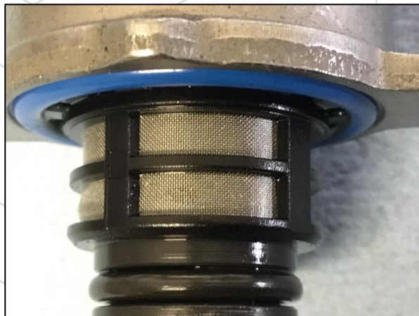
Figure 8: Clean FCA
